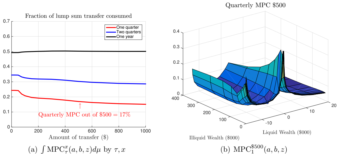
Figure 2: MPC Heterogeneity
